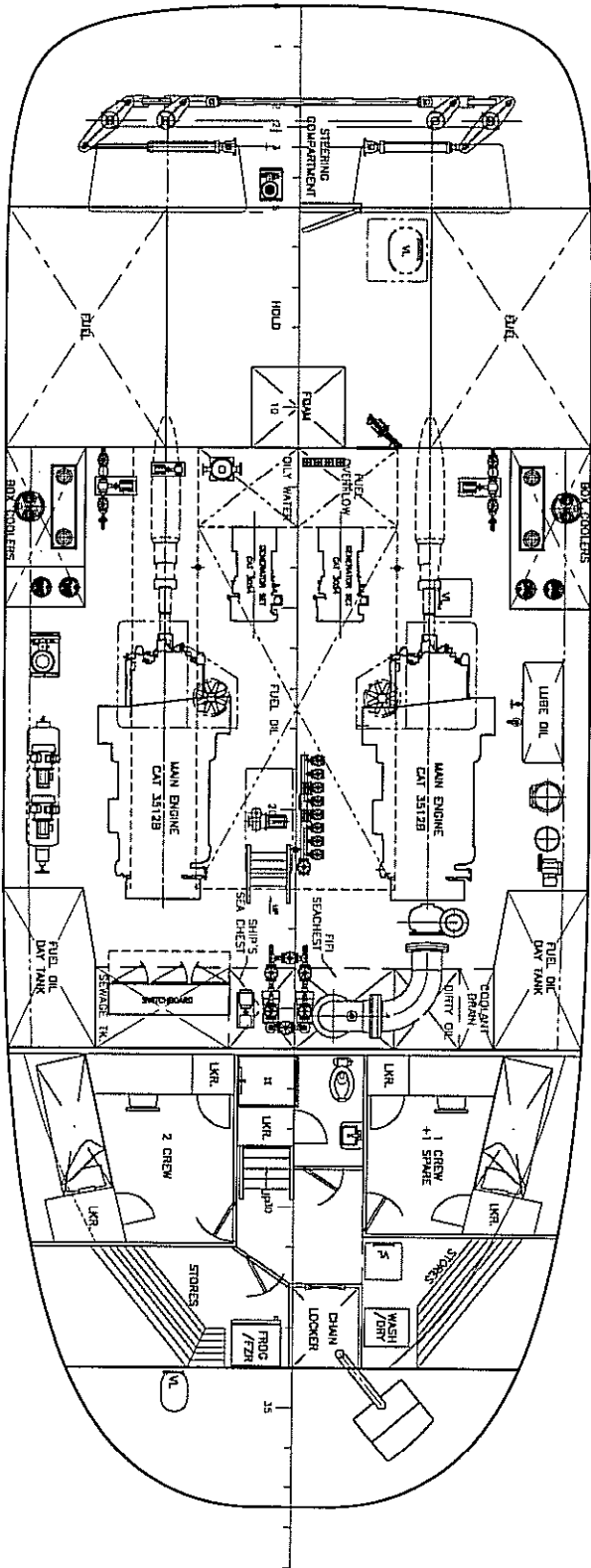
HOLD PLAN
