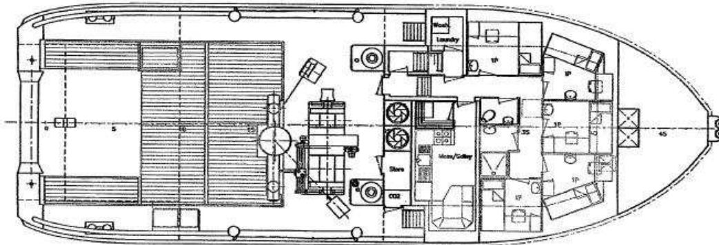
Below maindeck
